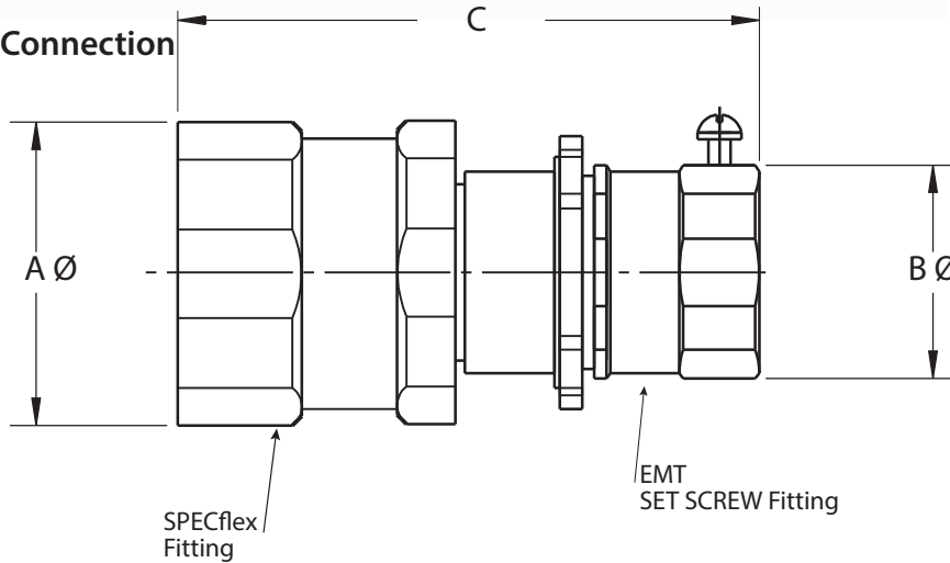
SPECflex EMT SET SCREW Adapters
